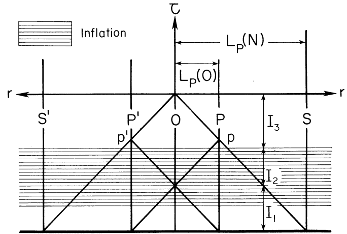
FIG. 2.—A conformal coordinate spacetime diagram of an inflationary Robertson-Walker universe. Inflation or any form of accelerated expansion (shown striated) in the early universe extends the range of conformal time prior to decoupling and transfers the particle horizon from world lines P, P' at distance L_p(0) to world lines S, S' at distance L_p(N) . When world line S is at a distance greater than 3 times that of world line P (and S' at a distance greater than 3 times that of P'), and hence L_p(N) > 3L_p(0) , the events p, p' that formerly were at the particle horizon of the standard universe (as shown in Fig. 1) are causally connected in the inflationary universe. Thus L_p(N) > 3L_p(0) is the sufficient condition that all events in the visible universe, such as d, d' in Fig. 1, are causally connected.
