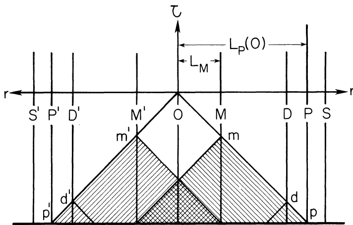
FIG. 1.—A conformal coordinate spacetime diagram of a standard Robertson-Walker universe that shows the observer's past light cone intersecting the vertical world lines of comoving bodies. Decoupling of the cosmic background radiation occurs on world lines, D, D' at events d, d'. World lines D, D' form the boundary of O's visible universe. The particle horizon L_P(0) on world lines P, P' forms the boundary of O's observable universe. World lines S, S' lie beyond the particle horizon and outside the observable universe. Events m, m' on world lines M, M' are seen in opposite directions at distance L_M ; when these world lines are at one-third the distance to the particle horizon, they are causally connected at maximum distance from the observer. Thus bodies in opposite directions at distances greater than L_P(0)/3 are causally unconnected.
