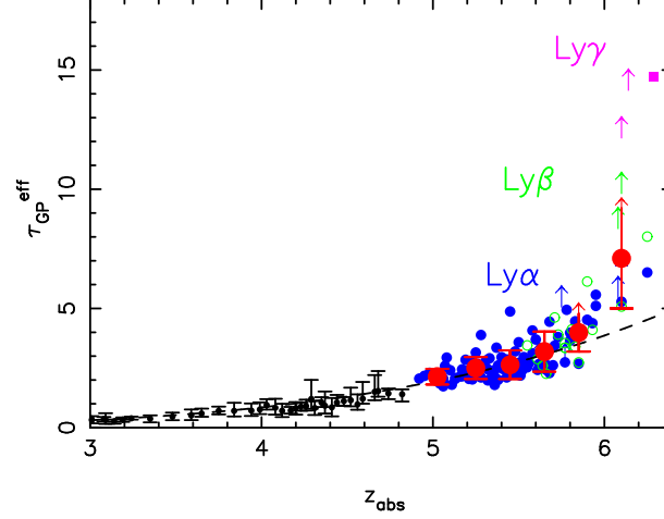
Fig. 5 Evolution of the Lyman \alpha , \beta and \gamma optical depth from the high redshift Sloan quasars. The Lyman \beta and Lyman \gamma restframe wavelengths are 1026 Å and 972.5 Å, respectively. The Lyman \beta measurements are converted to Lyman \alpha Gunn-Peterson optical depth using a conversion factor that reflects the difference in the cross section between the two transitions, which is a factor of 5.27 lower in the case of Lyman \beta (see [112, 38]). The values in the two highest redshift bins are lower limits, since they both contain complete Gunn-Peterson troughs. The dashed line shows a redshift evolution of \tau_\alpha \approx (1+z)^{4.3} . At z > 5.5 , the best-fit evolution has \tau_\alpha \approx (1+z)^{10.9} , indicating an accelerated evolution. The large filled symbols with error bars are the average and standard deviation of the optical depth at each redshift. The sample variance also increases rapidly with redshift. Figure taken from [60].
