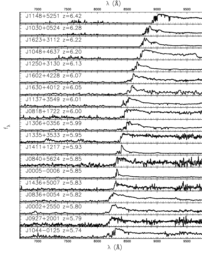
Fig. 4 Spectra for high redshift SDSS quasars. The Gunn-Peterson trough bluewards of the QSO Lyman \alpha emission that is clearly apparent in the highest redshift ones indicates that the Universe has become somewhat more neutral at these redshifts. A similar behavior is also seen bluewards of the QSO Lyman \beta region of the same spectra. The actual amount of increase in neutral hydrogen implied by these spectra is not clear [60].
