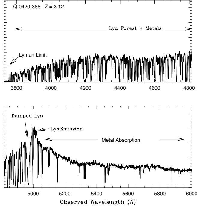
Fig. 3 High resolution spectrum of the z = 3.12 quasar Q0420-388 obtained with the Las Campanas echelle spectrograph by J. Bechtold and S. A. Sackett. The two panels cover the whole wavelength range of the spectrum. The Lyman \alpha forest is clearly indicated in the upper panel of the figure, bluewards of the quasar rest frame Lyman \alpha emission feature. Remember, at the rest frame this feature should have a wavelength of 1215.67 \text{ \AA} but since it is redshifted by a factor 1+z it appears at a wavelength of about 5000 \text{ \AA} . The Figure is courtesy of Jill Bechtold and appeared in [11].
