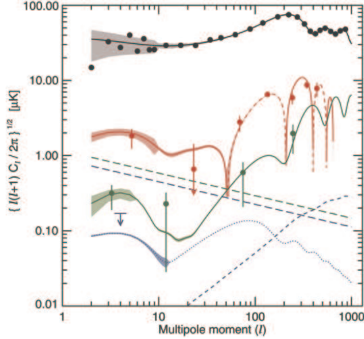
Fig. 9 The temperature and E-mode polarization power and cross-power spectra as measure by the WMAP satellite [152]. Plots of signal for TT (black), TE (red), and EE (green) for the best-fit model. The dashed line for TE indicates areas of anticorrelation. For more details about this Figure we refer the reader to the Page et al. [152]. Notice the excess power on large scales caused by reionization seen in the TE and EE power spectra.
