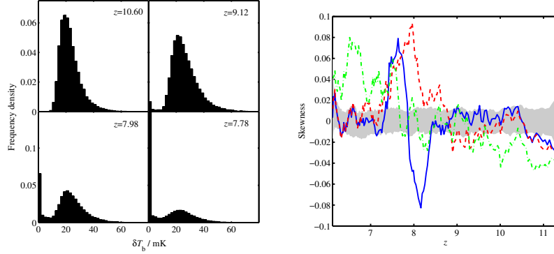
Fig. 25 Left hand panel: The distribution of \delta T_b in a certain cosmological simulation of reionization [90] at four different redshifts, showing how the PDF evolves as reionization proceeds. Note that the y-axis scale in the top two panels is different from that in the bottom two panels. The delta-function at \delta T_b = 0 grows throughout this period while the rest of the distribution retains a similar shape. The bar for the first bin in the bottom-right hand panel has been cut off; approximately 58 per cent of points are in the first bin at z = 7.78 [79]. Right hand panel: Skewness of the fitting residuals from data cubes with uncorrelated noise, but in which the residual image has been denoised by smoothing at each frequency before calculating the skewness. The three lines correspond to results from three different simulations [206, 90]. Each line has been smoothed with a moving average (boxcar) filter with a span of nine points. The grey, shaded area shows the errors, estimated using 100 realizations of the noise (see [79]).
