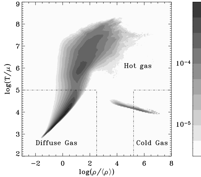
Fig. 10 The different baryon phases in the \rho - T diagram. Gray contours show a mass-weighted histogram: the baryon mass fraction at a given density and temperature. Each region corresponds to a given phase (diffuse background, hot, or cold gas) [161].
