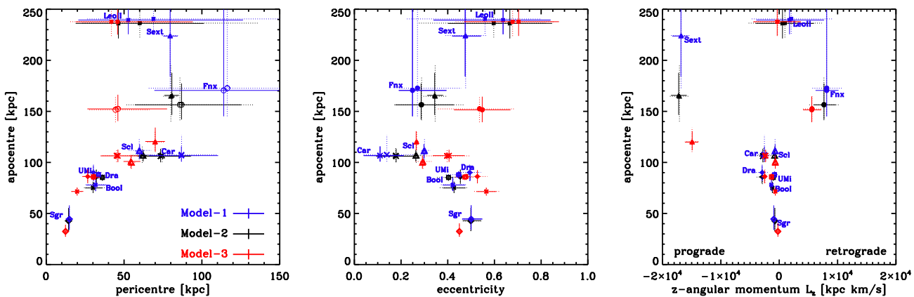
Fig. 22. Distribution of orbital parameters for the dSph. The different colours indicate computations with different potentials. The agreement is generally good, with Model-3 systematically leading to smaller pericentres as a result of its higher mass at the radii probed by the systems. Larger differences are found for the more distant objects, revealing the sensitivity of their orbits to variations in the assumed mass distributions for the Galaxy. The dSph eccentricity distribution differs from that shown in Fig. 20 for the globular clusters in our sample. The symbols with solid error bars correspond to the median and uncertainties derived using the Monte Carlo realisations, and those with dotted error bars also take a systematic error of 0.035 \text{ mas yr}^{-1} on each of the PM components into account.
