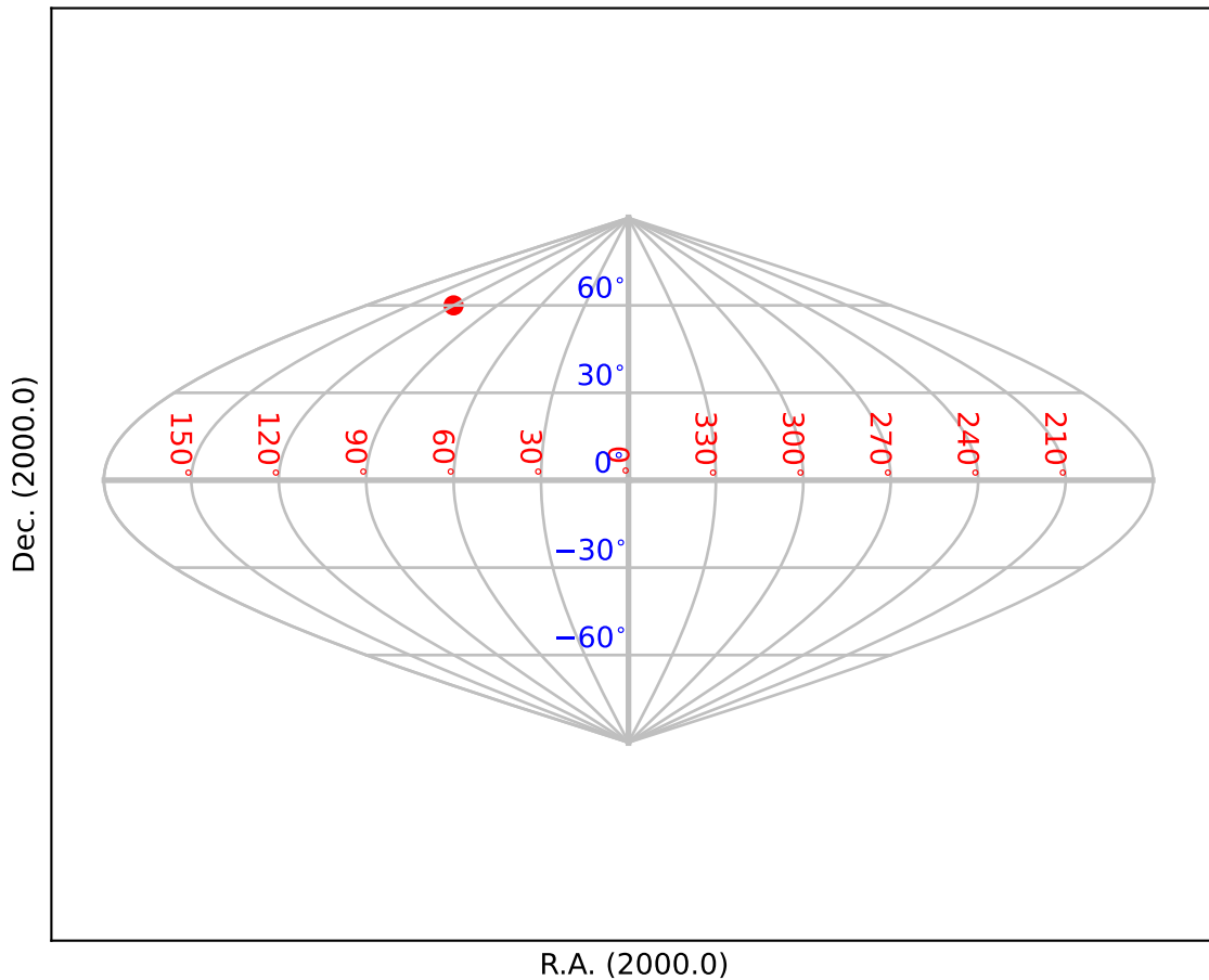
Fig. 16: Sanson-Flamsteed projection (SFL). (Cal. fig.20)
