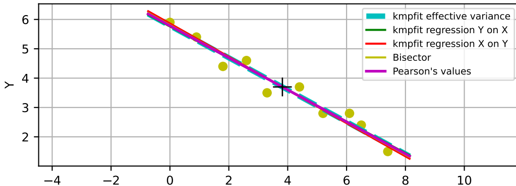
Pearson's data and model : y = a + b * x
