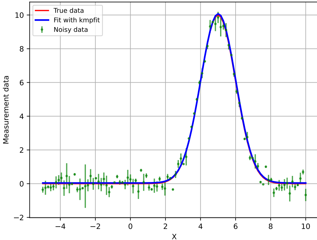
Least-squares fit to noisy Gaussian data using KMPFIT
