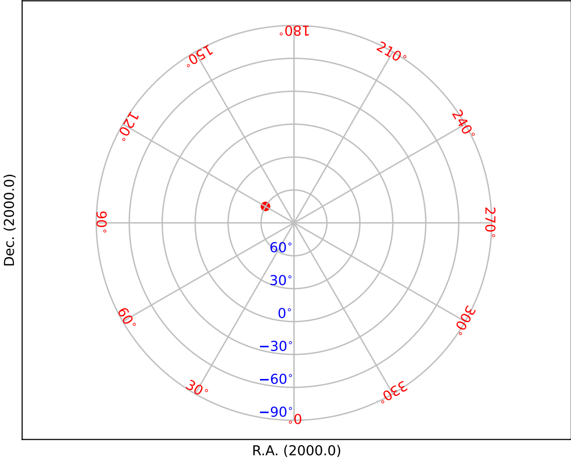
Fig. 8: Zenithal equidistant projection (ARC). (Cal. fig.11)
