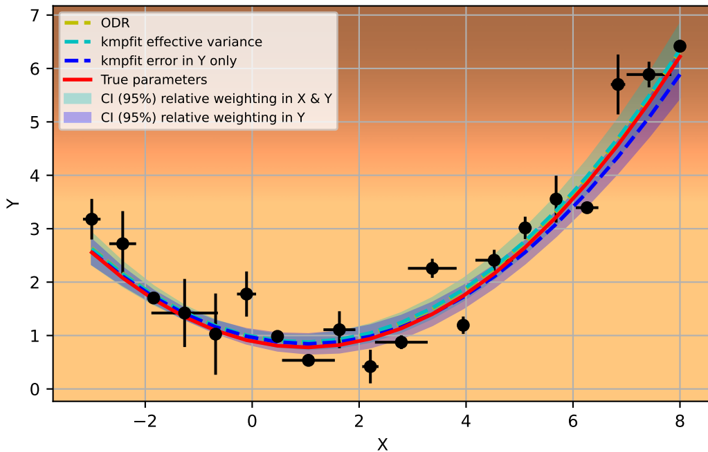
ODR and kmpfit with weighted fit. Model: y = a + bx + cx^2
