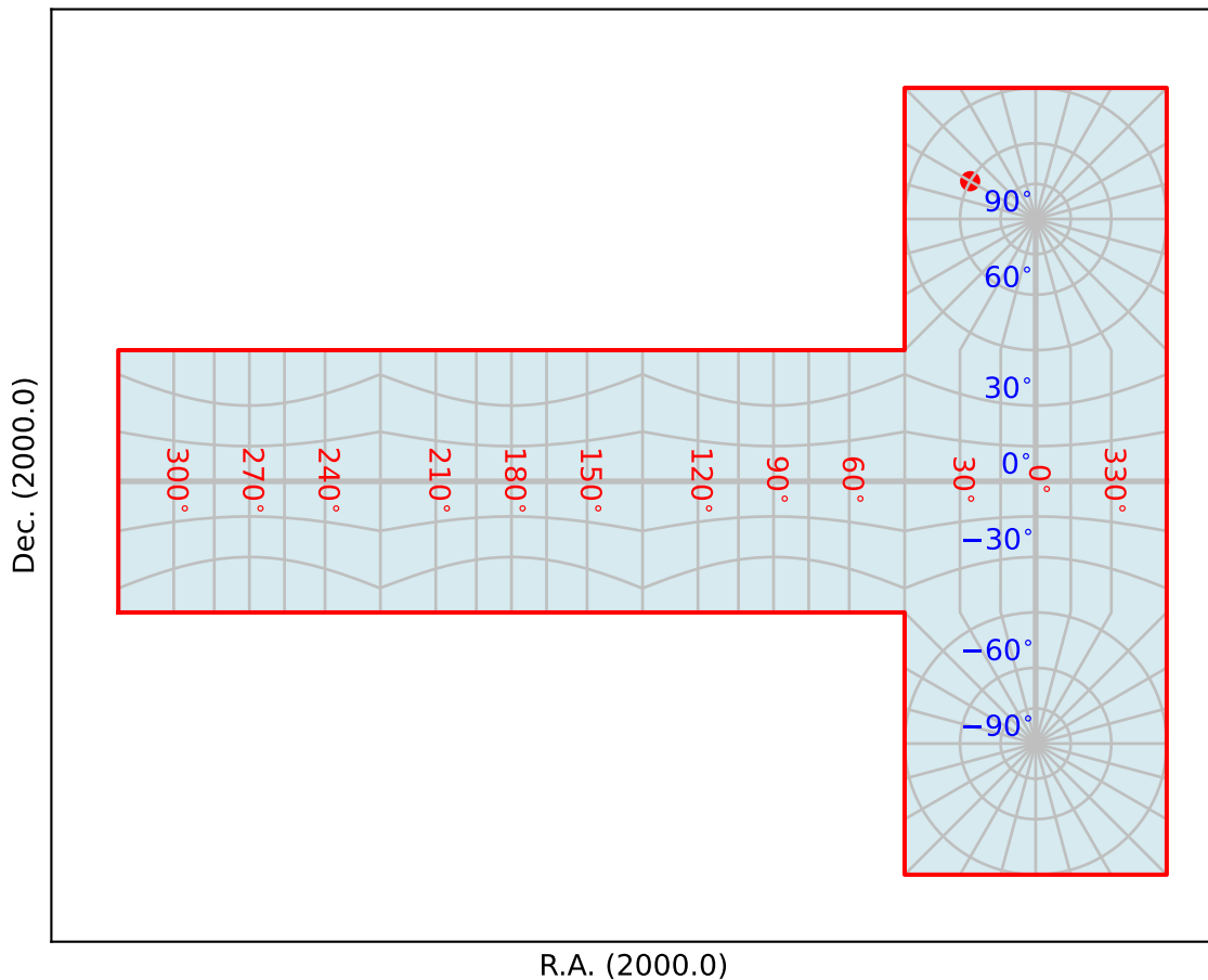
Fig. 26: Tangential spherical cube projection (TSC). (Cal. fig.30)
