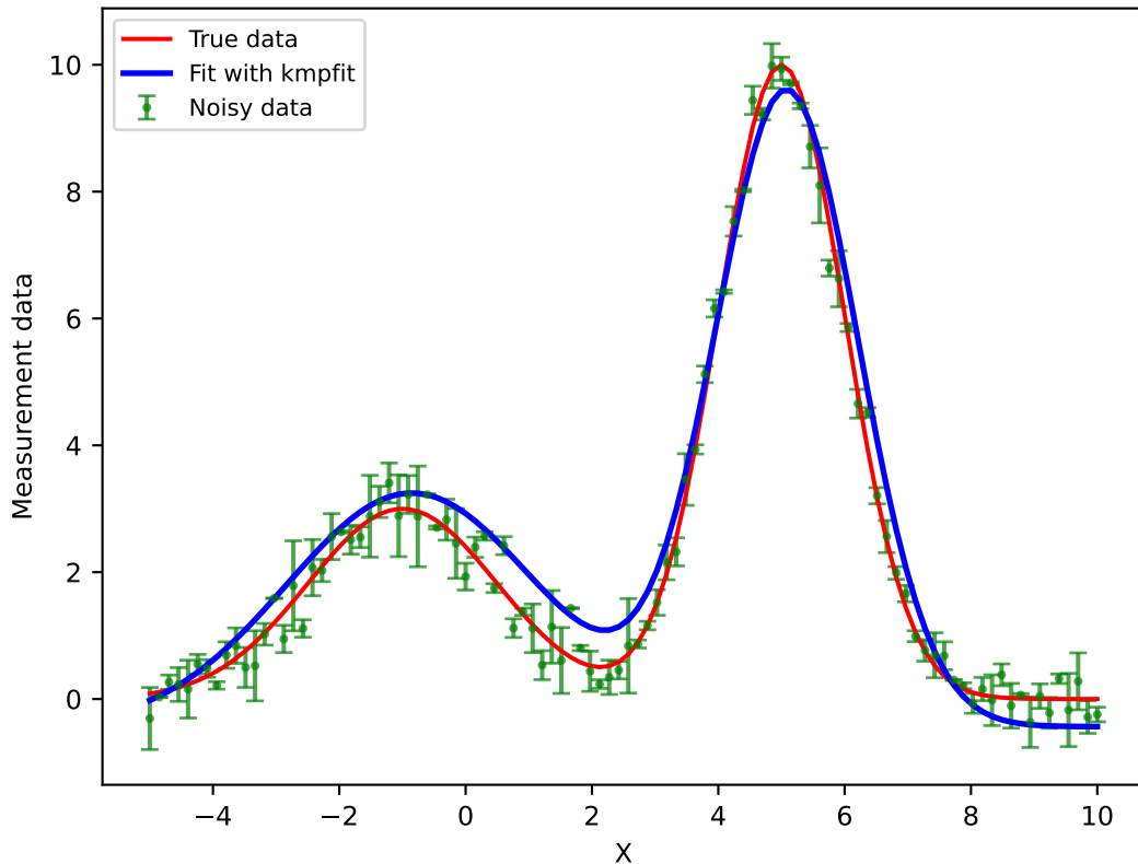
Least-squares fit to noisy multi-component Gaussian data
