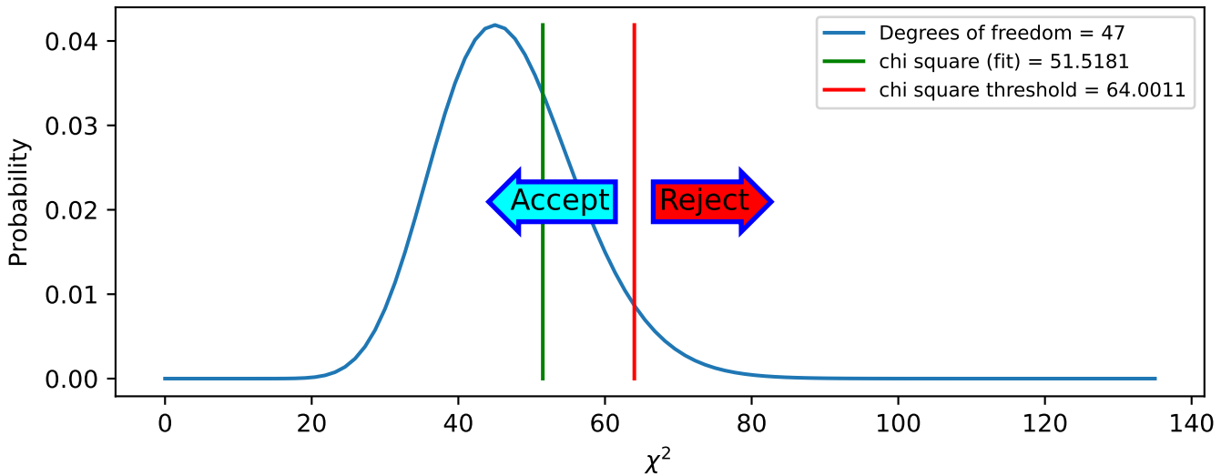
\chi^2 Probability density function for \nu = 47
