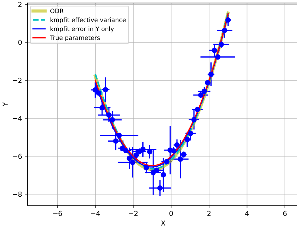
ODR and kmpfit with weighted fit. Model: y = a + bx + cx^2
