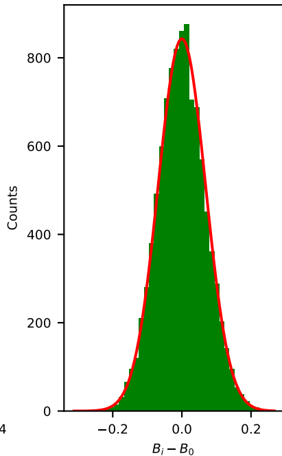
Distribution synthetic B
