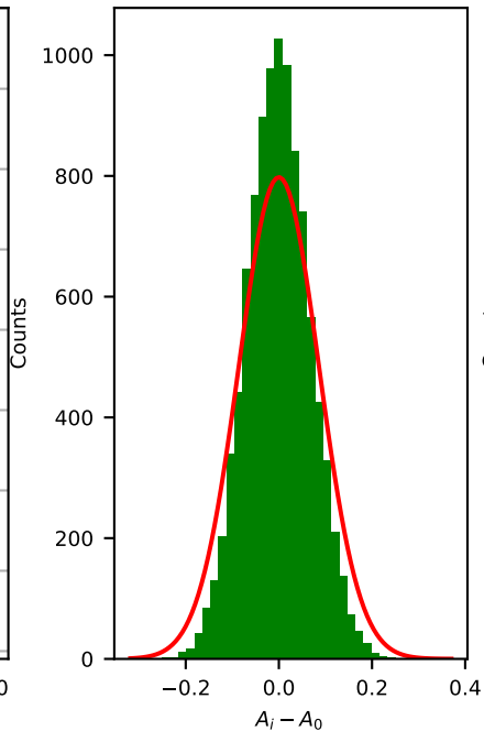
Distribution synthetic A
