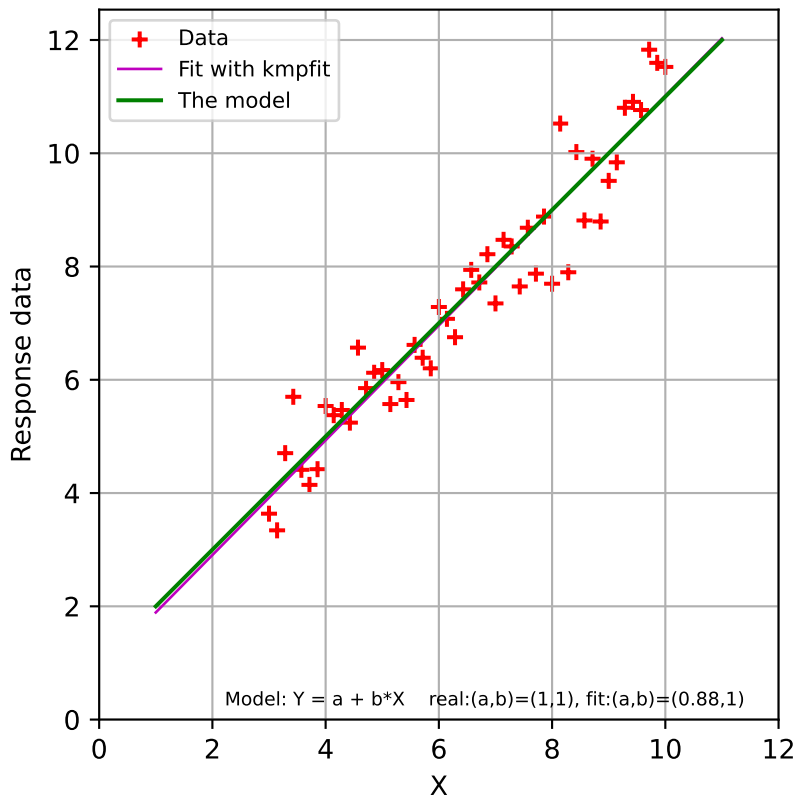
Least-squares fit to noisy data using KMPFIT
