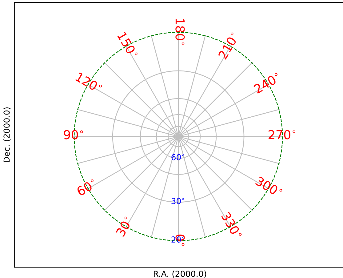
Gnomonic projection (TAN) diverges at \theta = 0^\circ . (Cal. fig.8)
