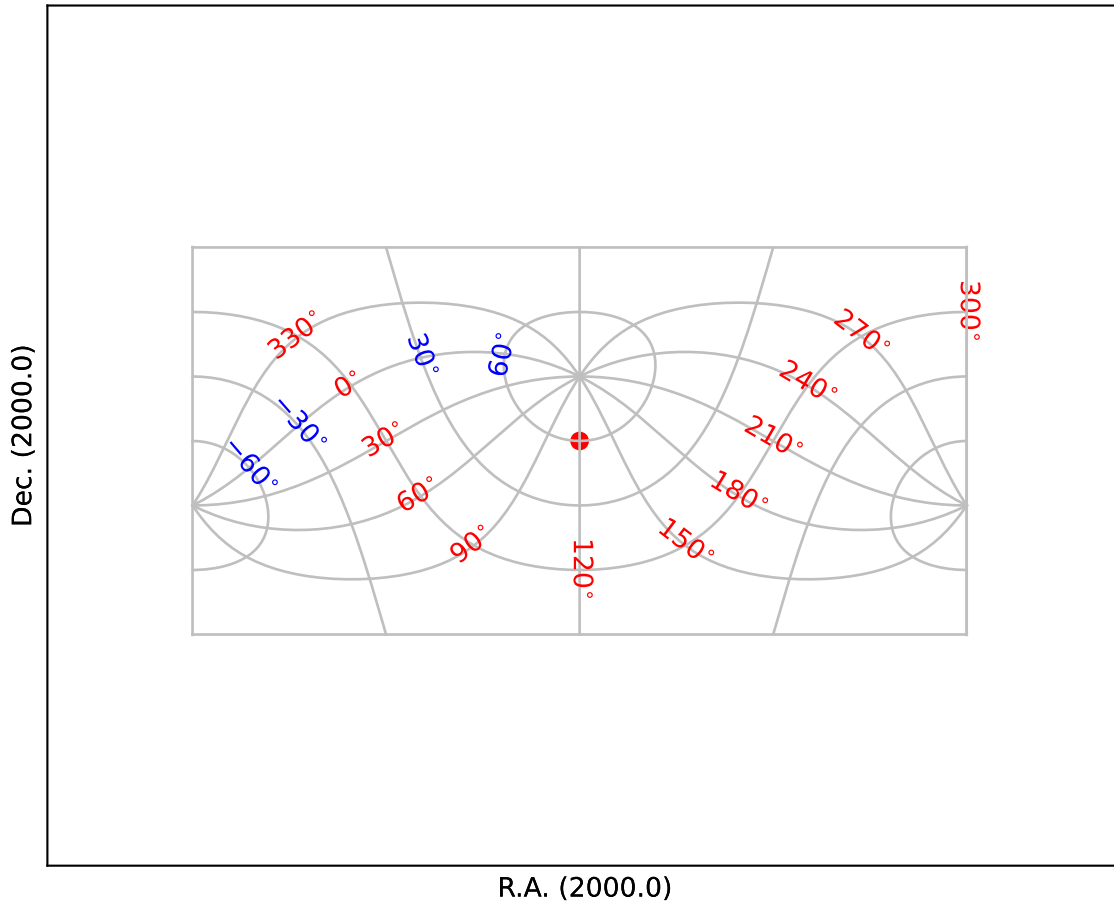
Fig. 1: Plate Carree projection (CAR), oblique with: (\alpha_0, \delta_0, \phi_p) = (120^\circ, 0^\circ, 0^\circ) and obviously cdelt1 > 0 . (Cal. fig. 2)
