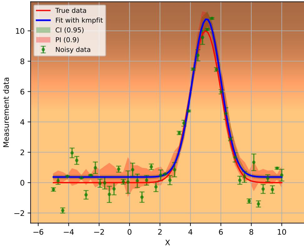
Confidence- and prediction bands for Gaussian model
