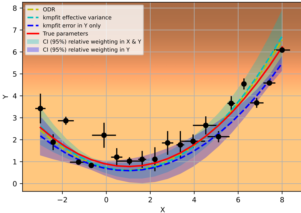
ODR and kmpfit with weighted fit. Model: y = a + bx + cx^2
