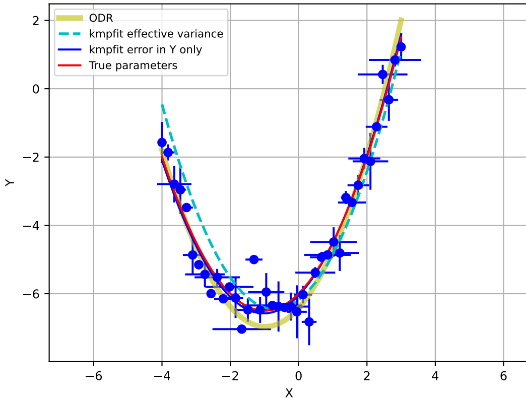
ODR and kmpfit with weighted fit. Model: y = a + bx + cx^2
