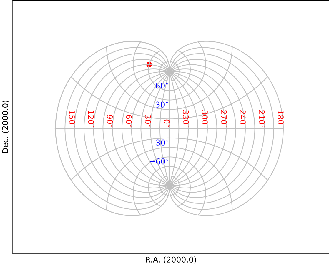
Fig. 25: Polyconic projection (PCO). (Cal. fig.29)
