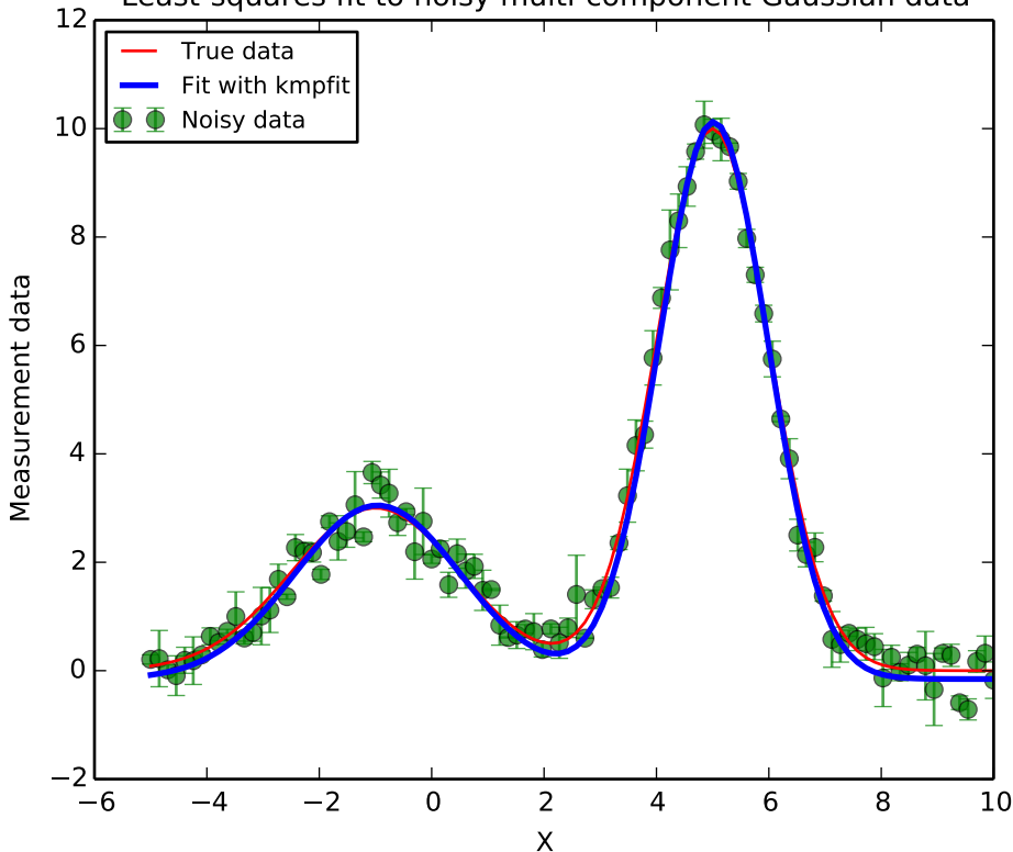
Least-squares fit to noisy multi-component Gaussian data
