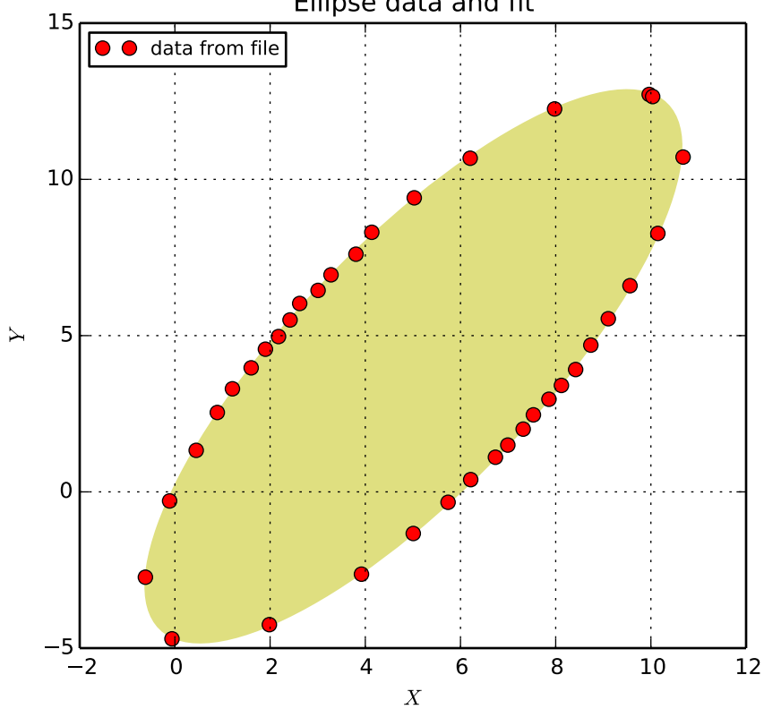
Ellipse data and fit
