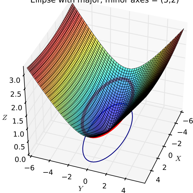
Ellipse with major, minor axes = (5,2)
