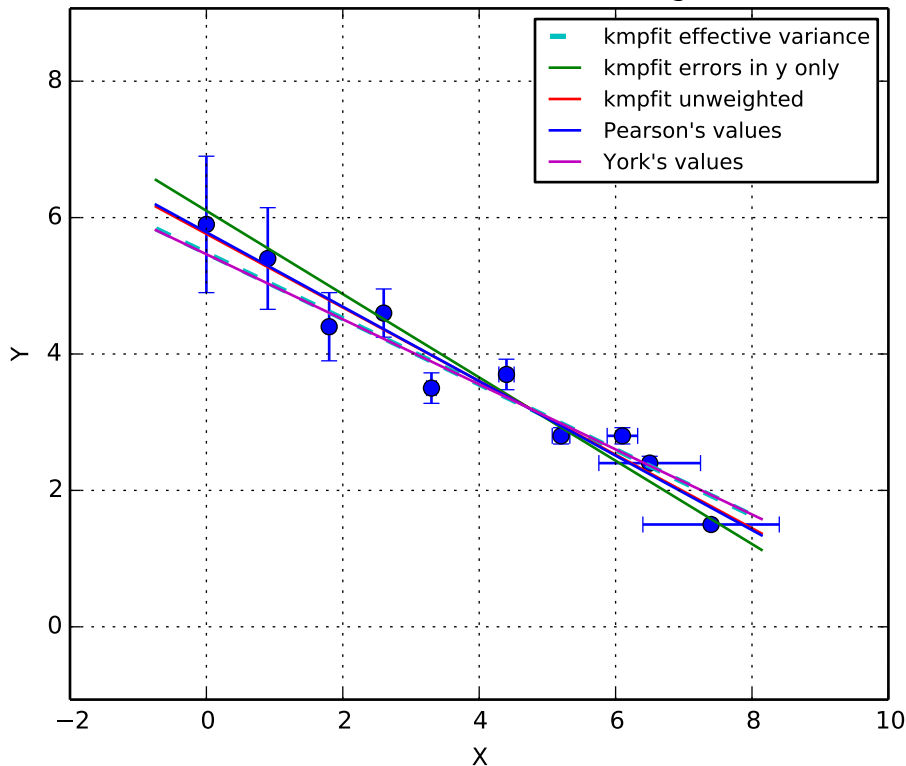
Pearson's data with York's weights
