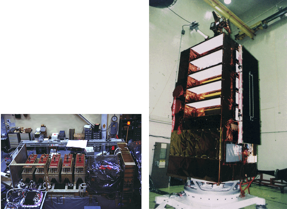
Figure 10: Left picture shows the assembly of the RXTE, the right picture shows the RXTE when it was complete.[10]
