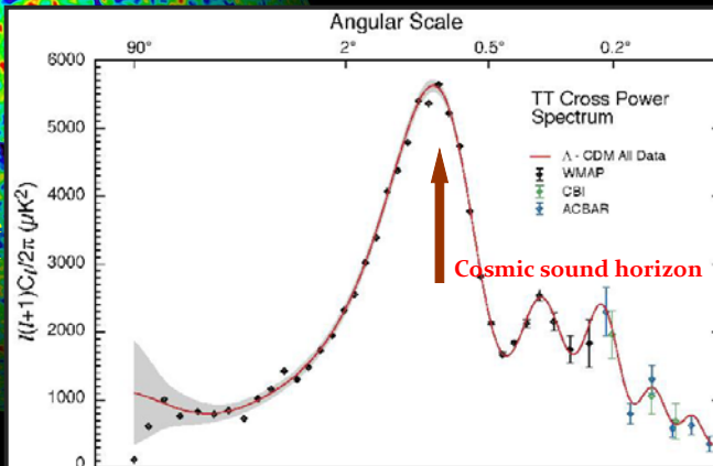
The WMAP CMB temperature power spectrum
