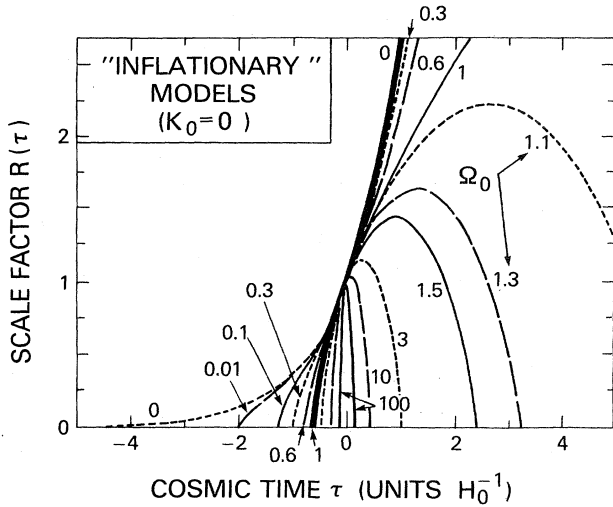
FIG. 2. "Inflationary" Friedmann \tau models. The family of scale factors R(\tau) for models satisfying the "inflationary constraint" (three-space curvature K_0=0 ). The free parameter, shown on the curves, is \Omega_0 . The cosmological constant \Lambda is determined from \Omega_0 by Eq. (14).
