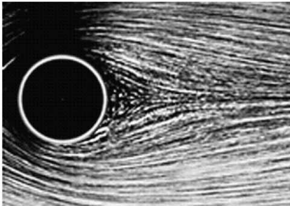
Re = 9.6
