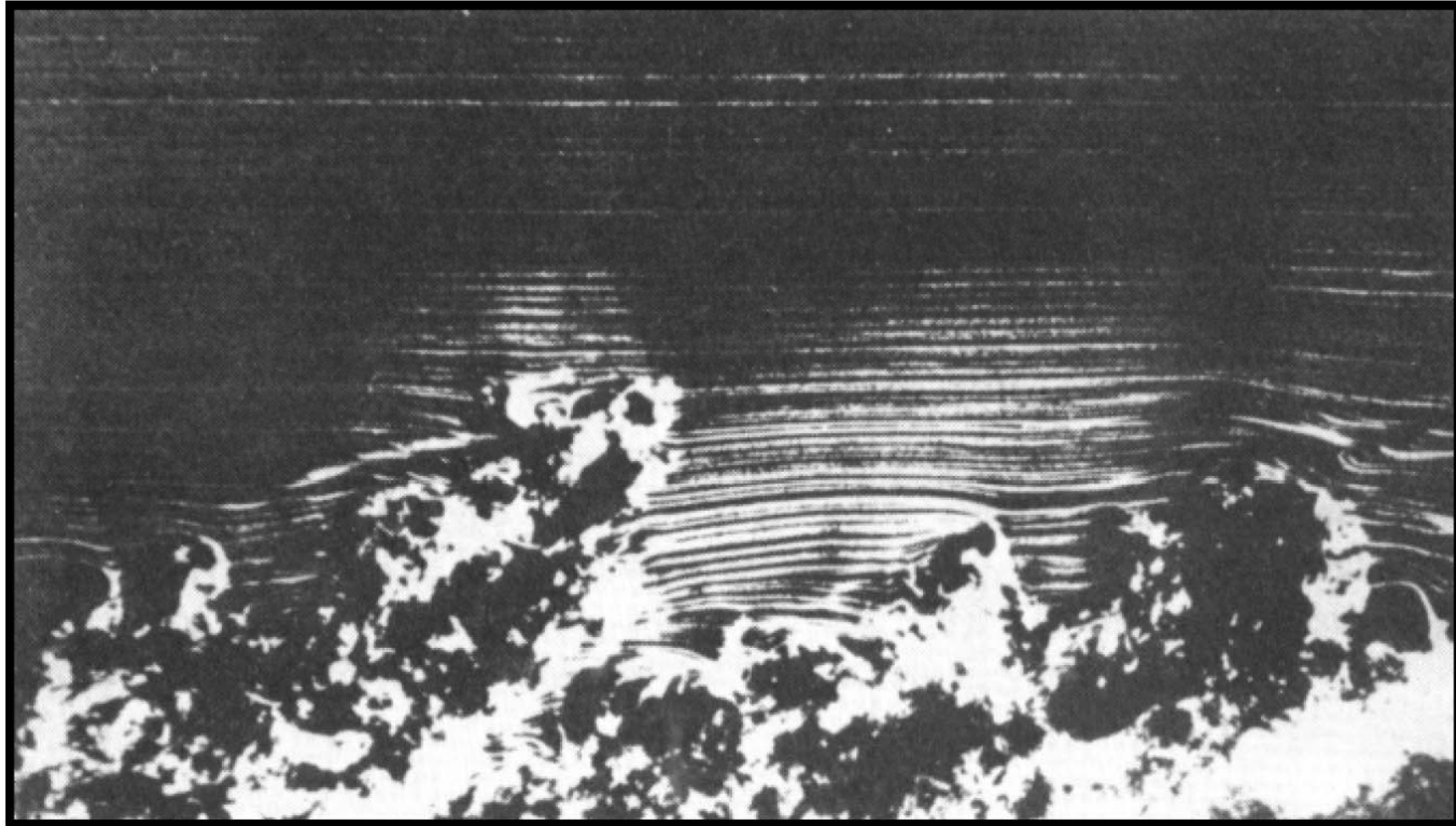
Close-up view of the turbulent boundary layer.
