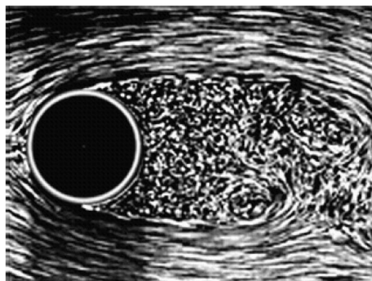
Re = 2000
