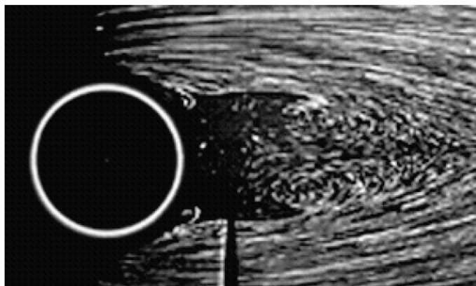
Re = 30.2
