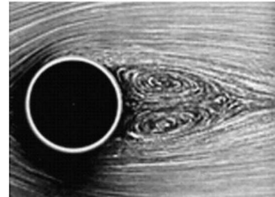
Re = 26
