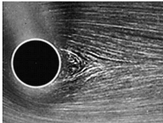
Re = 13.1
