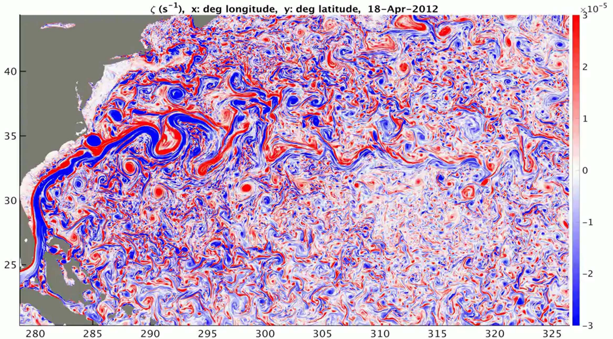
Simulation turbulent Gulfstream flow (Ocean Motion)
