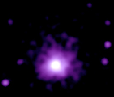
CL J1226.9+3332
