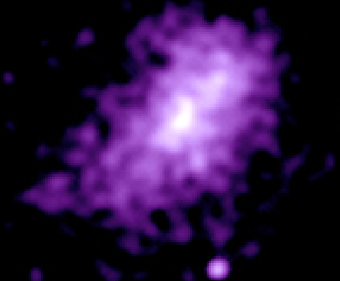
MACS J1149.5+223
