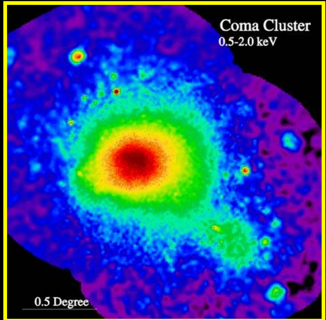
ROSAT X-ray image Coma Cluster
