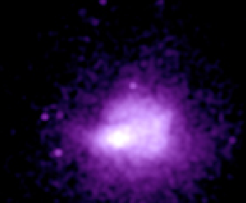
Abell 1914
