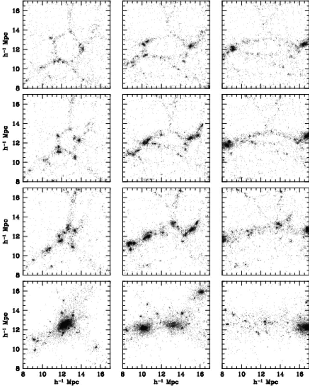
Figure 4. Three examples (left to right) of the void-in-cloud process in action in numerical simulations of structure formation in a SCDM scenario ( \Omega_0 = 1.0 , h_0 = 0.5 ). Top to bottom panels show the evolution of the particle distribution in comoving coordinates from early to late times (resp. a = 0.3, 0.4, 0.5 and 1.0 , the current epoch). The initially underdense regions are crushed by the collapse of the overdense regions which surround them. The void in the first row of 4 panels shows a nearly spherical collapse sequence. The other two rows involve configurations involving more anisotropic surrounding matter distributions (and force fields).
