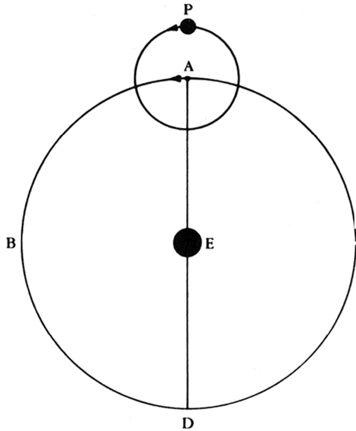
epicycle (basic)
