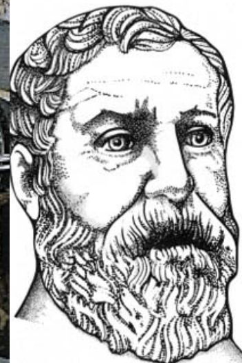
Aristarchus
