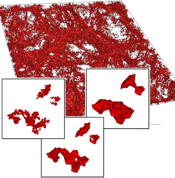
FIG. 3.— Top: \alpha shape of a GIF ACDM simulation, slice through simulation box. Bottom: \alpha shape at 3 different values of \alpha .
