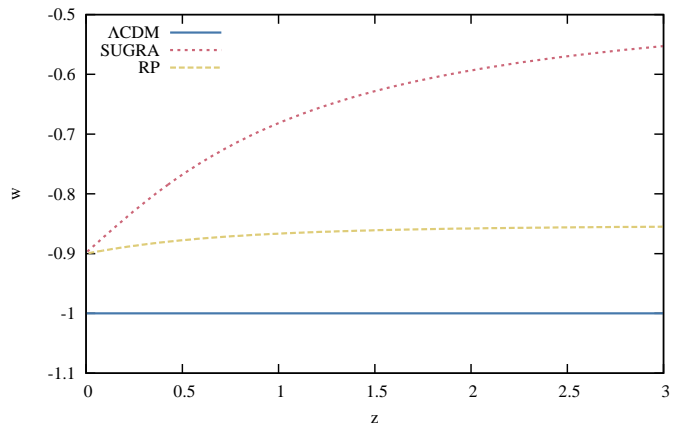
FIG. 4.— Evolution of the dark energy equation of state parameter w(z) for ACDM (solid), SUGRA (dotted) and RP (dashed).
