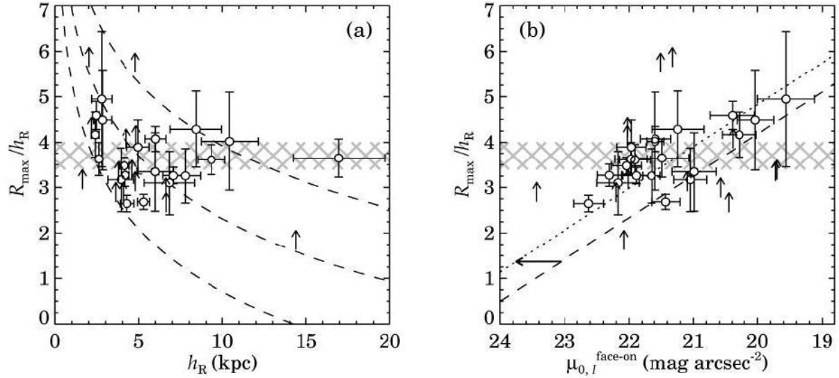
Figure 11: Correlations of R_{\max}/h with scalelength h and face-on central surface brightness \mu_{0,\text{fo}} for a sample of edge-on galaxies. The cross-hatched regions show the prediction from a collapse model as in van der Kruit (1987) and Dalcanton et al. (1997); the dotted and dashed lines show predictions from the star formation threshold model of Schaye (2004) for three different values of the disk mass. (from Kregel & van der Kruit, 2004b, ; see there for details of the models.)
