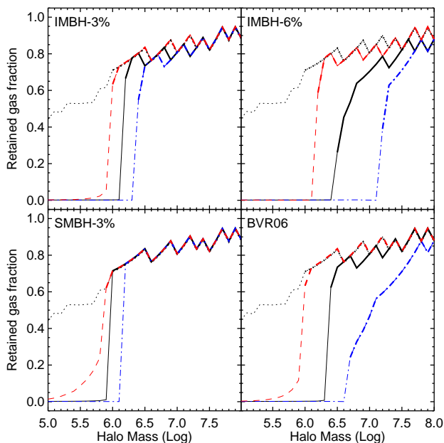
Figure 12. Fraction of gas retained by a halo at the end of our simulations in halos virializing at z_{vir} = 10 , as a function of the total halo mass. The order of the panels and the meaning of the continuous, dashed and dot-dashed lines are the same as in Fig. 2; the dotted lines refer to the unperturbed model. The thickness of the line indicates whether a certain halo mass is below (thin line) or above (thick line) the critical mass. The seesaw behavior for high masses is purely numerical (i.e. due to the discrete number of shells).
