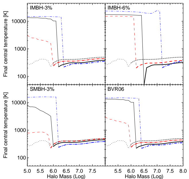
Figure 13. Central gas temperature at the end of our simulations in halos virializing at z_{vir} = 10 , as a function of the total halo mass. The order of the panels and the meaning of the continuous, dashed and dot-dashed lines are the same as in Fig. 2; the dotted lines refer to the unperturbed model. The thickness of the line indicates whether a certain halo mass is below (thin line) or above (thick line) the critical mass.
