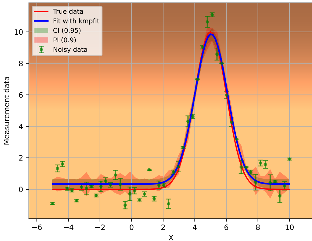
Confidence- and prediction bands for Gaussian model
