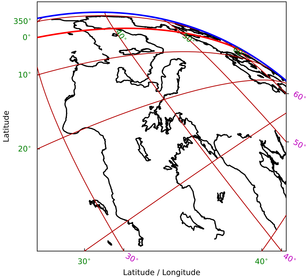
Fig. 36: Earth in zenithal perspective (AZP). (Cal. fig.36)
