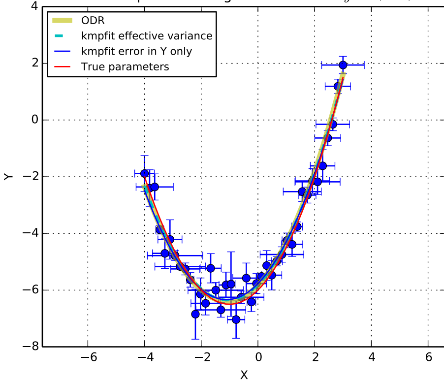
ODR and kmpfit with weighted fit. Model: y = a + bx + cx^2
