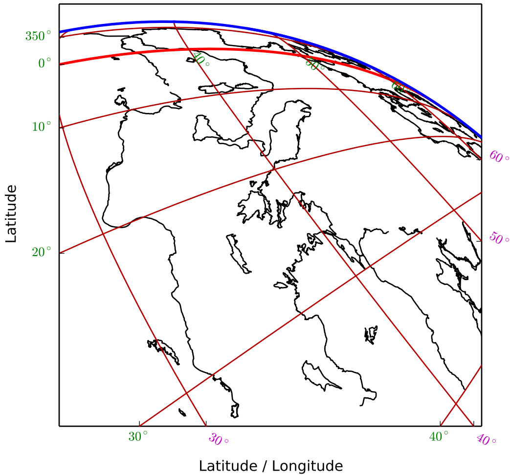
Fig. 36: Earth in zenithal perspective (AZP). (Cal. fig.36)
