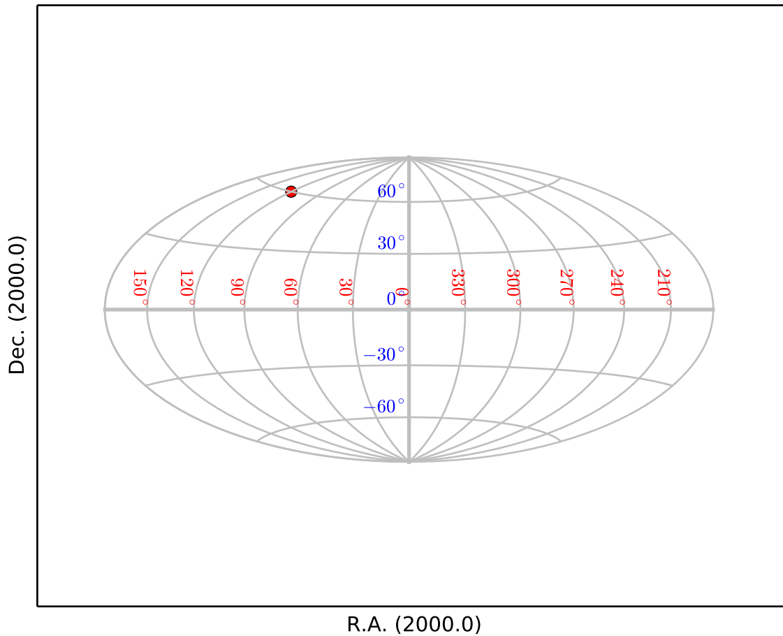
Fig. 19: Hammer Aitoff projection (AIT). (Cal. fig.23)
