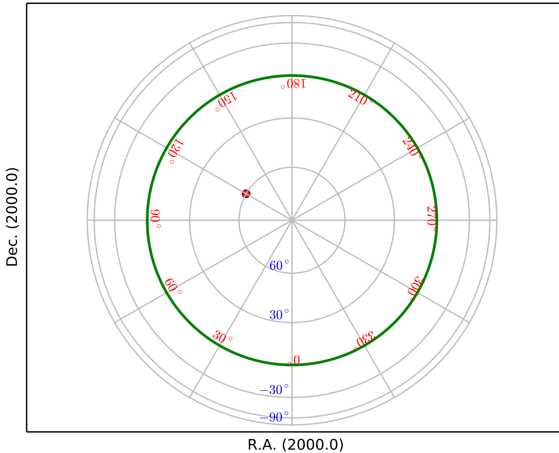
Fig. 10: Zenith equal area projection (ZEA). (Cal. fig.13)
