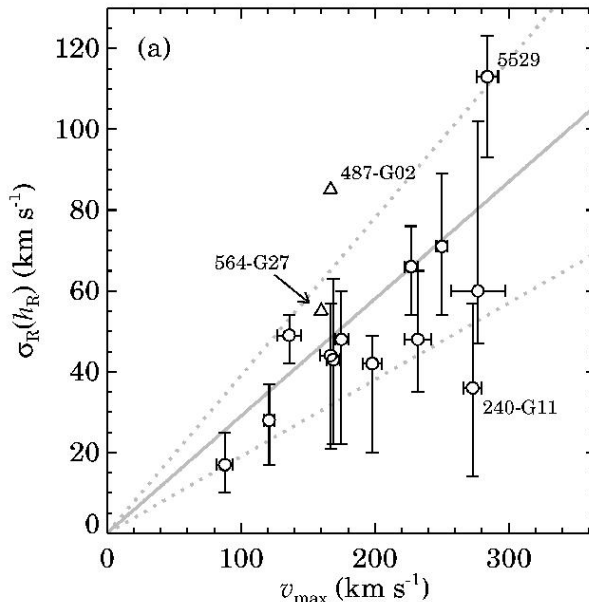
Figure 4: Stellar disk velocity dispersion, measured at one scalelength in edge-on galaxies versus the maximum rotational velocity. The gray lines indicate the relation \sigma_R(h) = (0.29 \pm 0.10) V_{\text{rot}} (Bottema, 1993). (From Kregel, van der Kruit & Freeman, 2005)
