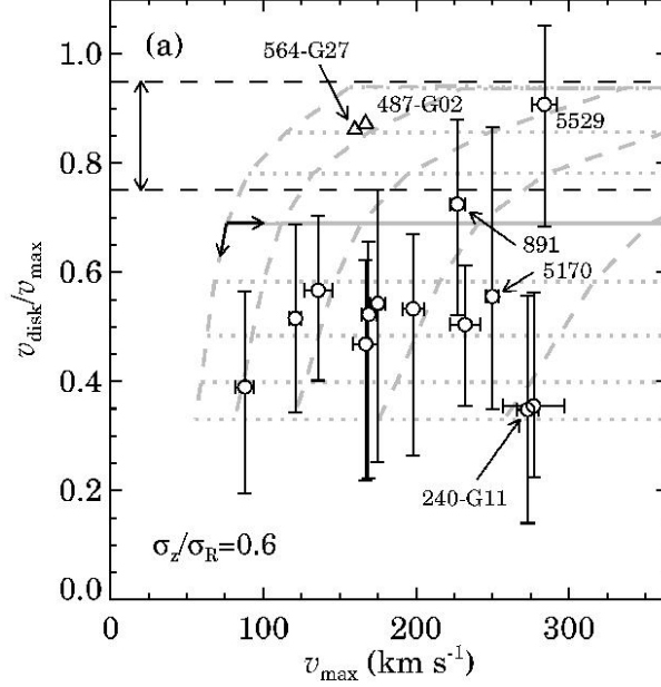
Figure 6: The contribution of the disk to the amplitude of the rotation curve V_{\text{disk}}/V_{\text{rot}} for a sample of 15 edge-on galaxies as a function of the rotation velocity itself. The horizontal dashed lines are the limits of 0.85 \pm 0.10 from Sackett (1997), which would indicate Fmaximal disks. The axis ratio of the velocity ellipsoid is assumed to be 0.6. The grey lines correspond to collapse models of Dalcanton et al. (1997); dashed lines connect models of the same total mass ( \log_{10}(M_{\text{tot}}) = 10 - 13 in steps of 0.5) and dotted lines connect models with the same spin parameter (logarithmically spaced, separated by factors of 0.2 dex, with the solid line at \lambda = 0.06 ). The arrows indicate the direction of increasing M_{\text{tot}} and \lambda . The two galaxies without error bars are the same ones as the outliers in fig. 5. (From Kregel, van der Kruit & Freeman, 2005)
