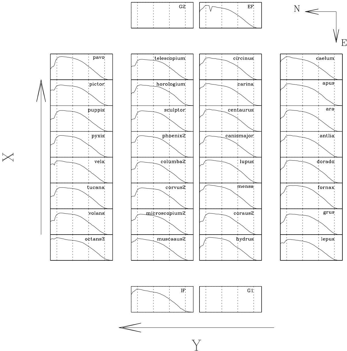
Figure 10: The QE curves for all CCDs in the mosaic, laid out as the mosaic itself. The solid curve in each panel is the measured QE for that device; the dotted curve is the average for all 32 science CCDs. The wavelength range from 320 to 1100nm is plotted; dotted lines indicate 400, 600, 800 and 1000nm. X and Y are coordinates in the focal plane; for the default instrument rotator position angle of 0 X points West and Y points North. To be updated?
