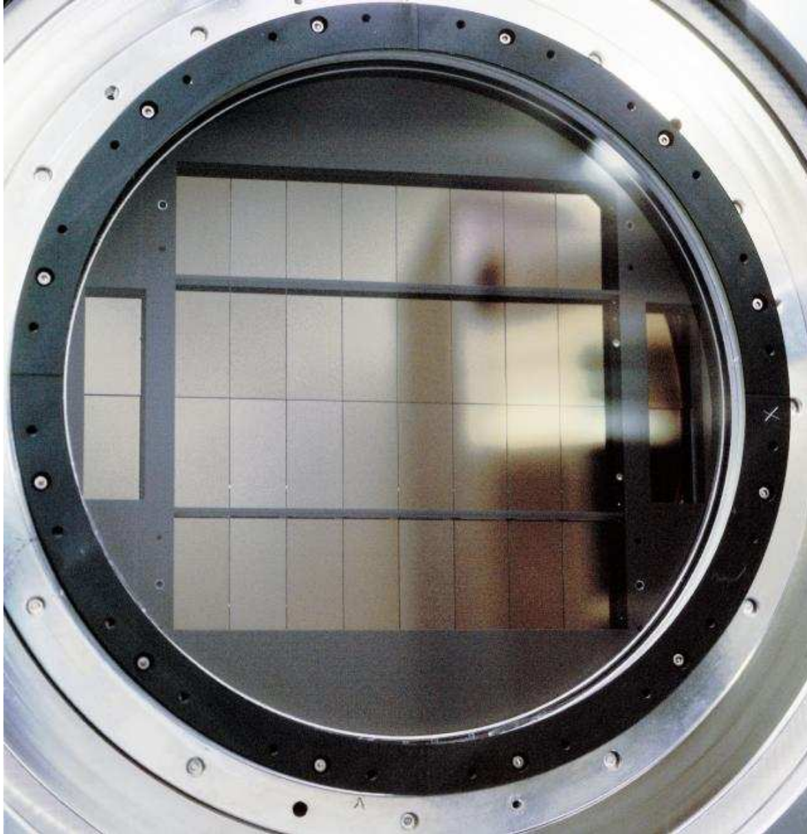
Figure 4: The layout of the 32 science CCDs and the four auxiliary CCDs in the focal plane. The science array covers a 1 degree x 1 degree area of sky, with 16k x 16k pixels of 0.21 arcsec. All CCDs fit inside a circle of diameter 1.4 degrees on the sky.
