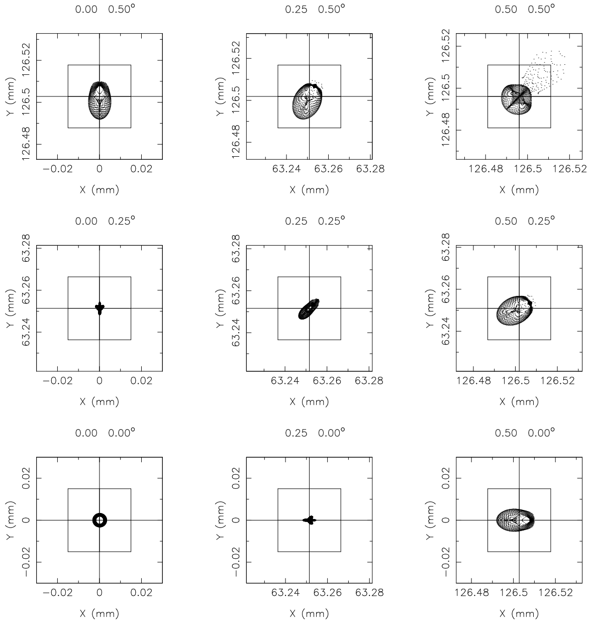
Figure 3: Sample spot diagrams for 500nm light in the OmegaCAM focal plane. A 2x2 pixel grid ( 30\mu\text{m} \times 30\mu\text{m} , corresponding to 0.43'' ) is shown as well.
