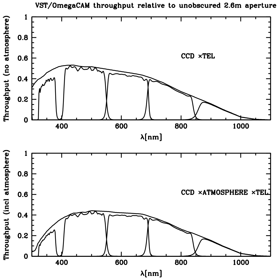
Figure 7: Throughput of the VST / OmegaCAM / CCDs, excluding and including atmospheric absorption (airmass zero and one). The sensitivity of the system including the five Sloan filters is also shown. To be updated with real measurements.
