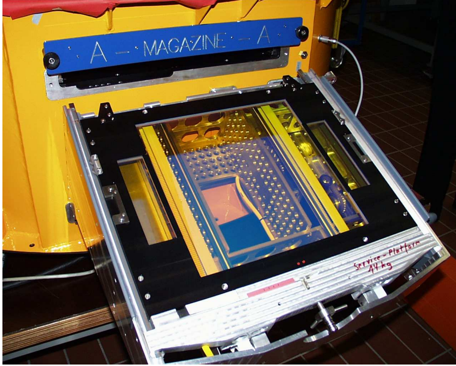
Figure 5: A single OmegaCAM filter ready to be loaded into the instrument. Note the separate filters covering the auxiliary CCDs.
